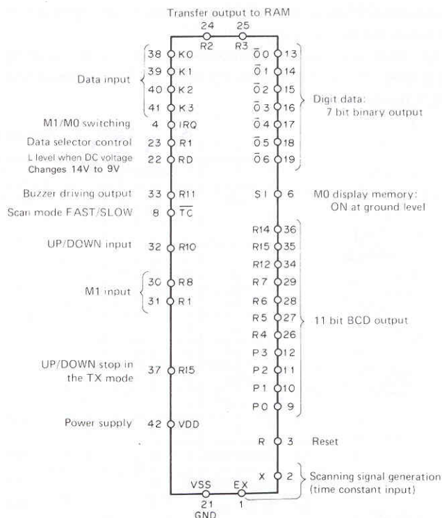
Fig. 14 Microprocessor explanation
